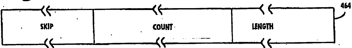
Fig. 7F SP WRITE DMA LENGTH (R/W)
